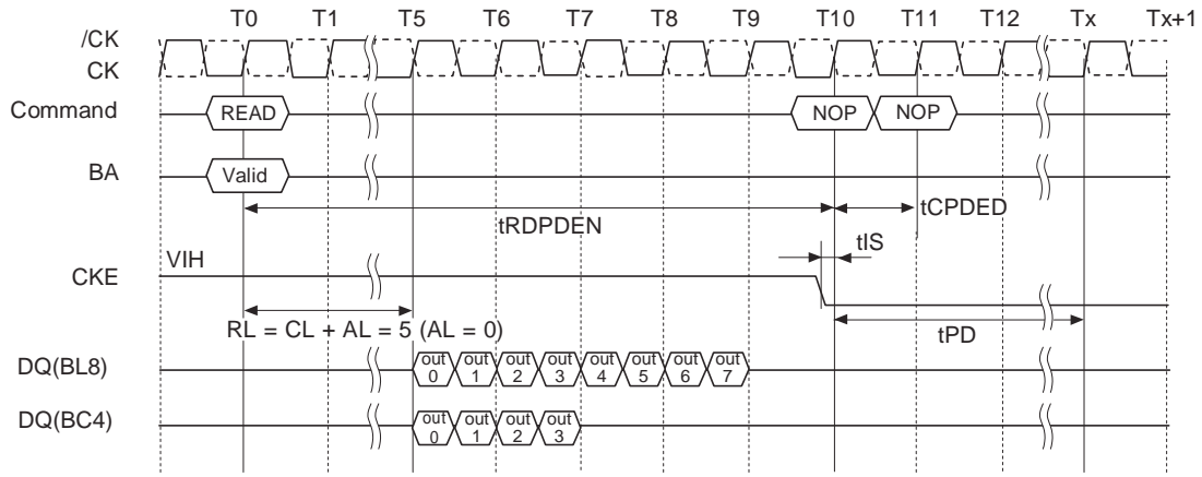
Power-Down Entry after Read and Read with Auto Precharge
