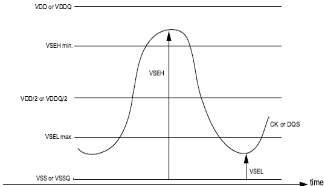
Single-Ended Requirement for Differential Signals.
