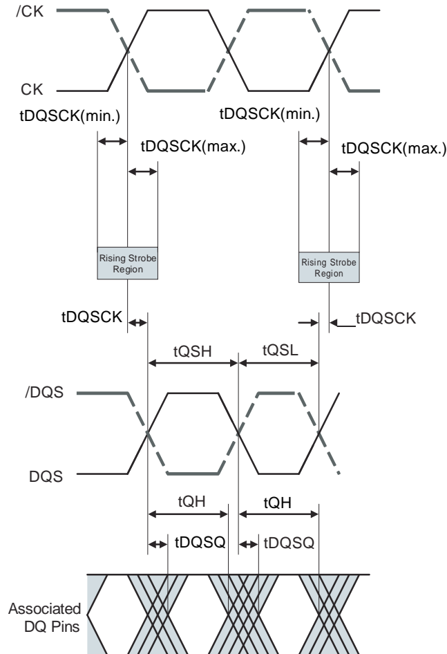
Read Timing Definition
