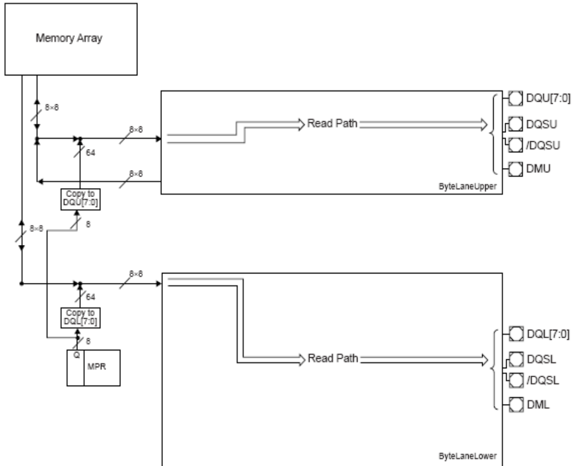
Functional Block Diagram of Multi Purpose Register in x16 DDR3 SDRAM
