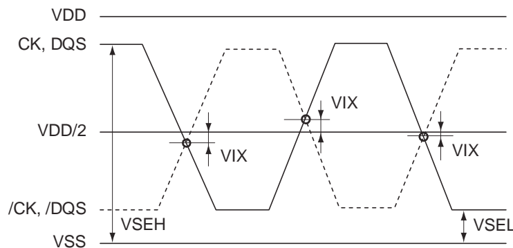
VIX Definition
