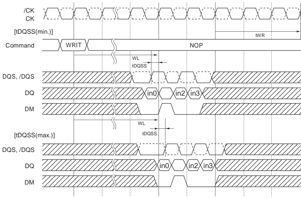
Data Mask Function, WL = 5, AL = 0 shown
