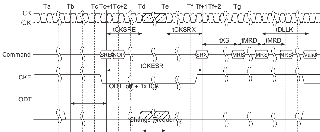
DLL Switch Sequence from DLL-Off to DLL-On
